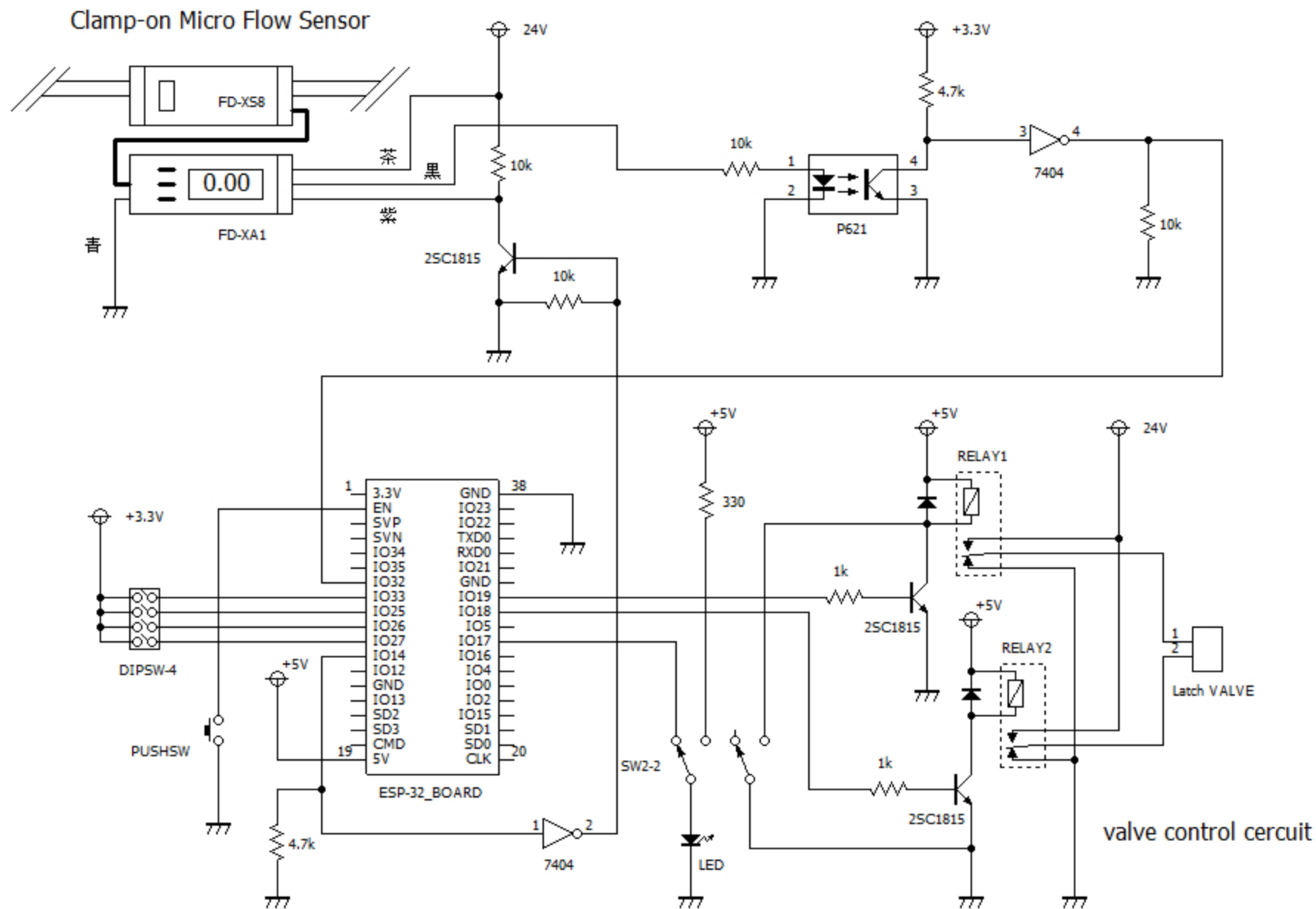
Automatic meterd water supply system for monkey cages
